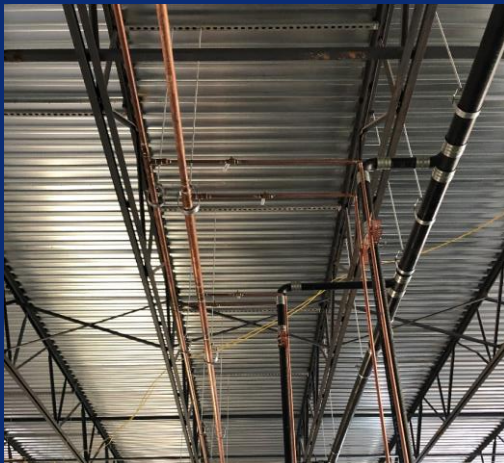
Lower level O/H plumbing lines installed
